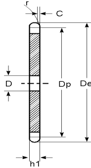
CONVEYOR SERIES-CARRIER ROLLER DUPLEX PITCH-2060/C2060
