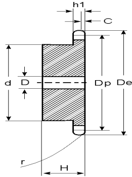
CONVEYOR OR DRIVE SERIES-STANDARD ROLLER DUPLEX PITCH-2050/C2050
