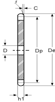
CONVEYOR SERIES-CARRIER ROLLER DUPLEX PITCH-2080/C2080
