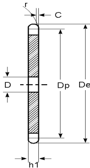
CONVEYOR SERIES-CARRIER ROLLER DUPLEX PITCH-2050/C2050
